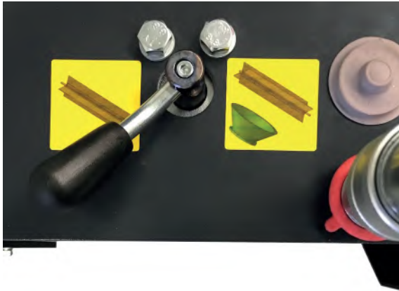
Main/side brush activation lever
