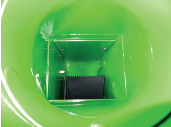
Replaceable housing liner and turbine made of HARDOX steel
